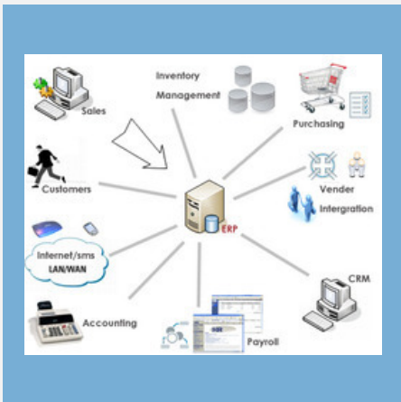
ERP Software
